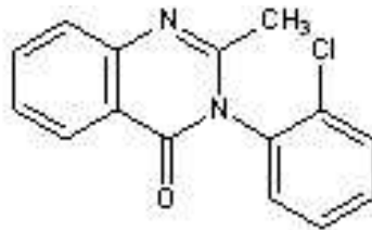
Mecloqualone C_{15}H_{11}ClN_2O
