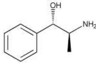
Cathine, C_{12}H_{16}N_2O
